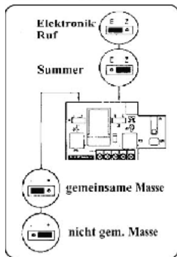
Jumper Positionen
